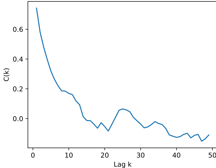
LUMO Autocorrelation
