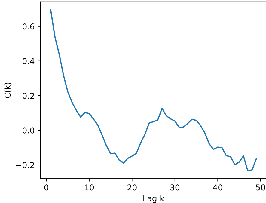
GAP Autocorrelation
