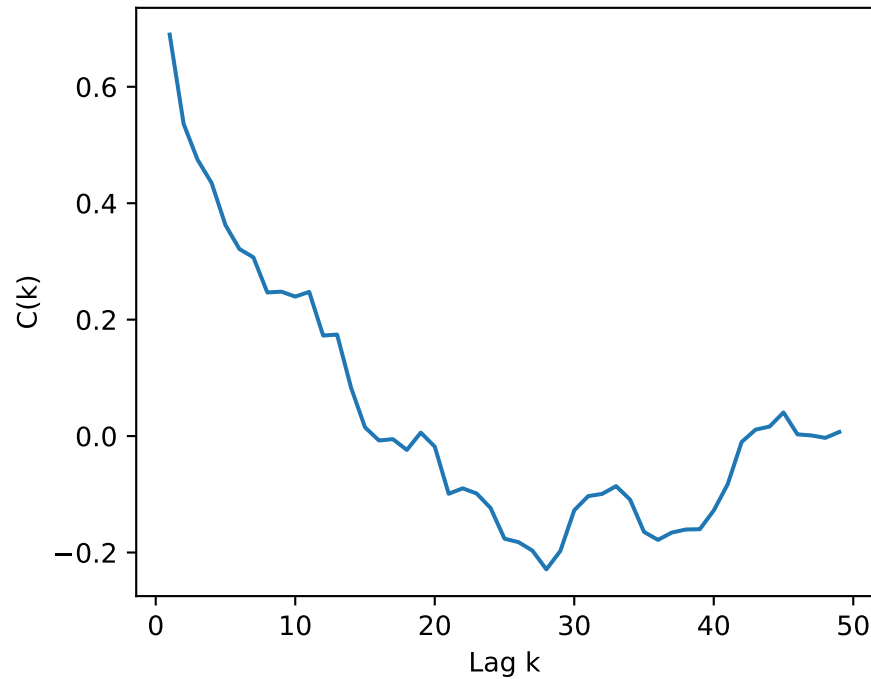
HOMO Autocorrelation
