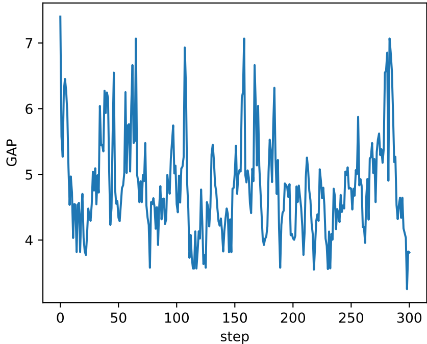
GAP - evolution
